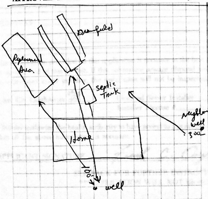
APPROVED PLANS S, Marsh Creek Rd → N
